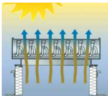
functions SMOKEJET®/SMOKEJET® D: fair weather ventilation and SHEV systems
